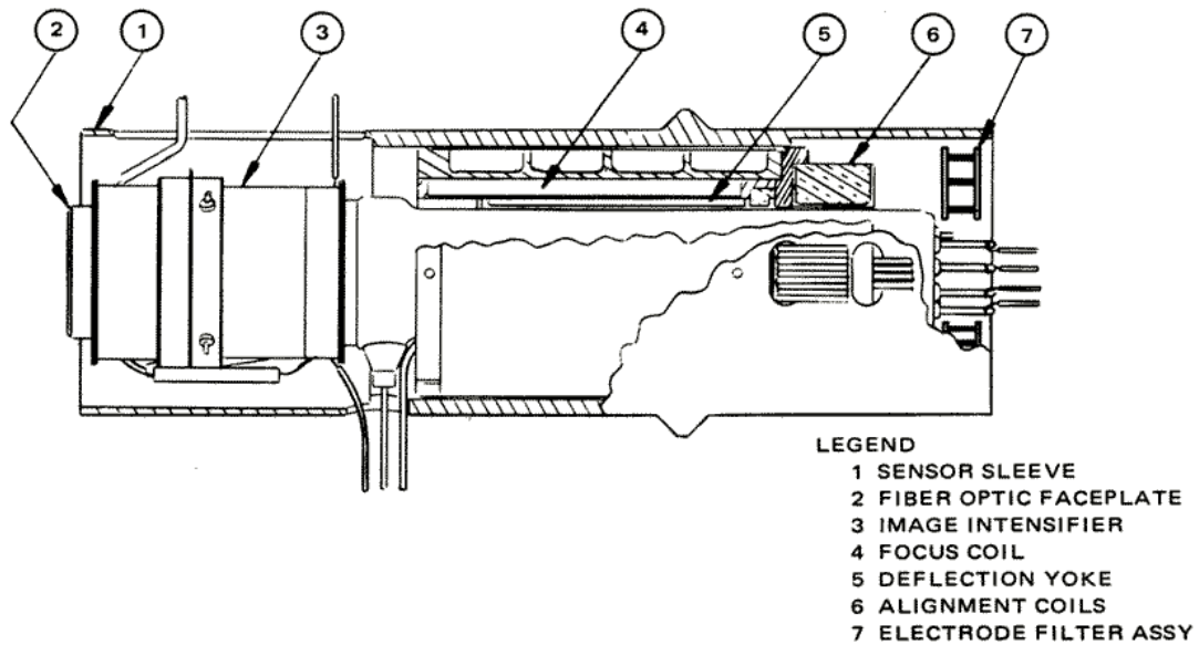
Figure 1-11. CTV Camera Sensor Assembly
