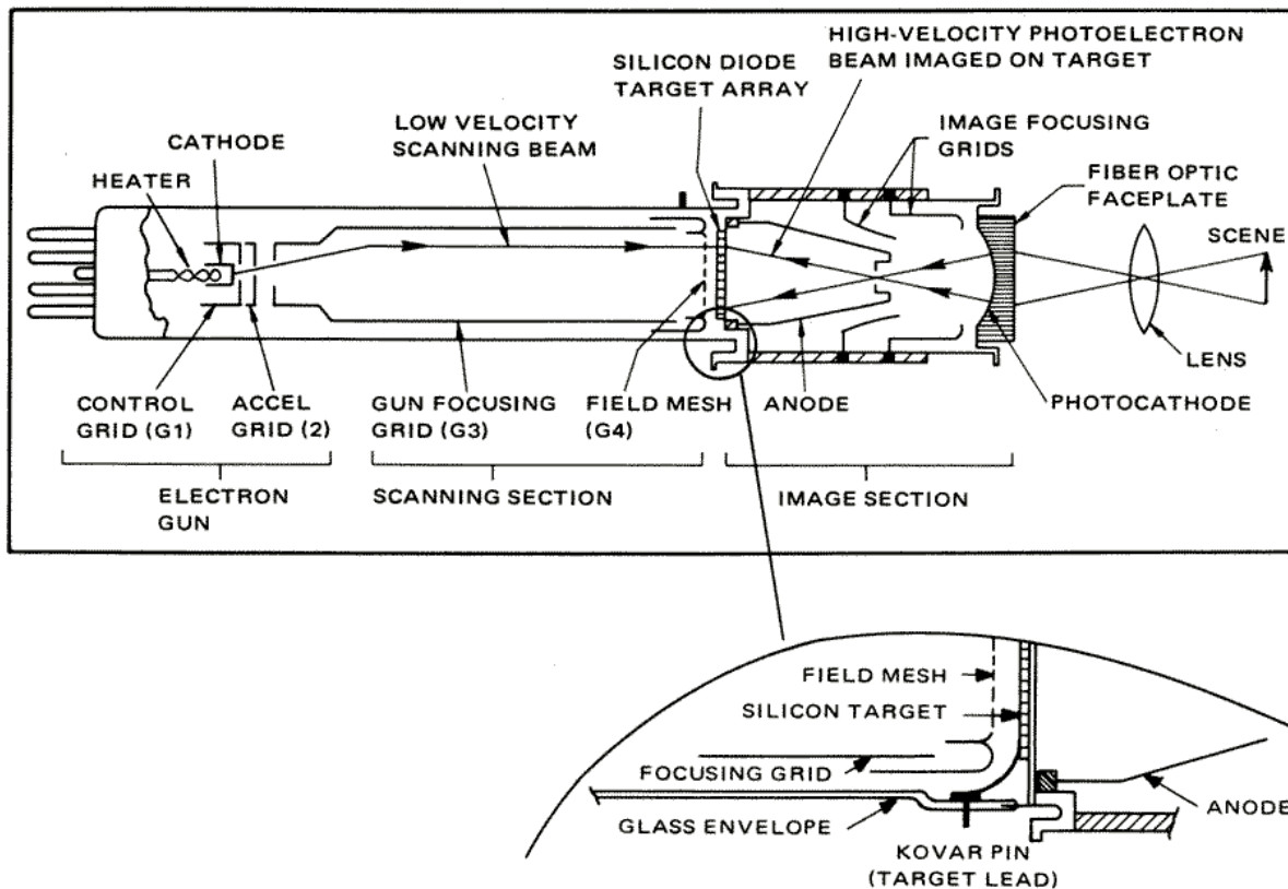
Figure 1-12. Sectional View of the SIT Sensor
