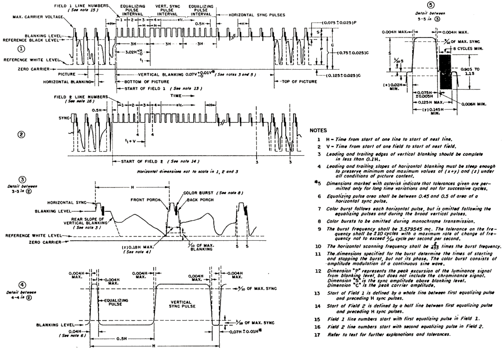
Figure 1-20. FCC Television Synchronizing Waveform (Color)
